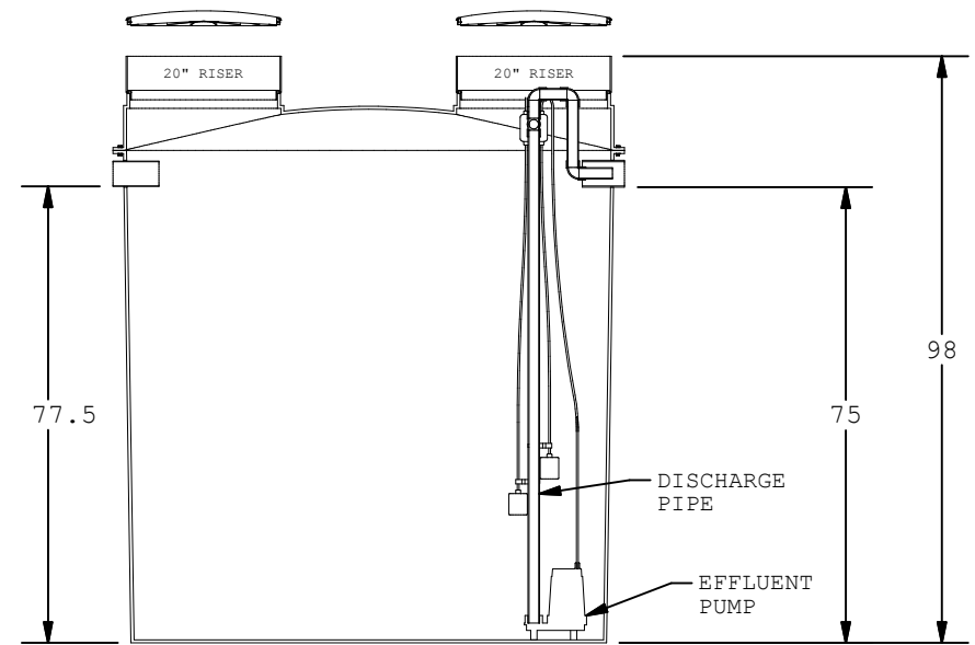
PUMP TANK
