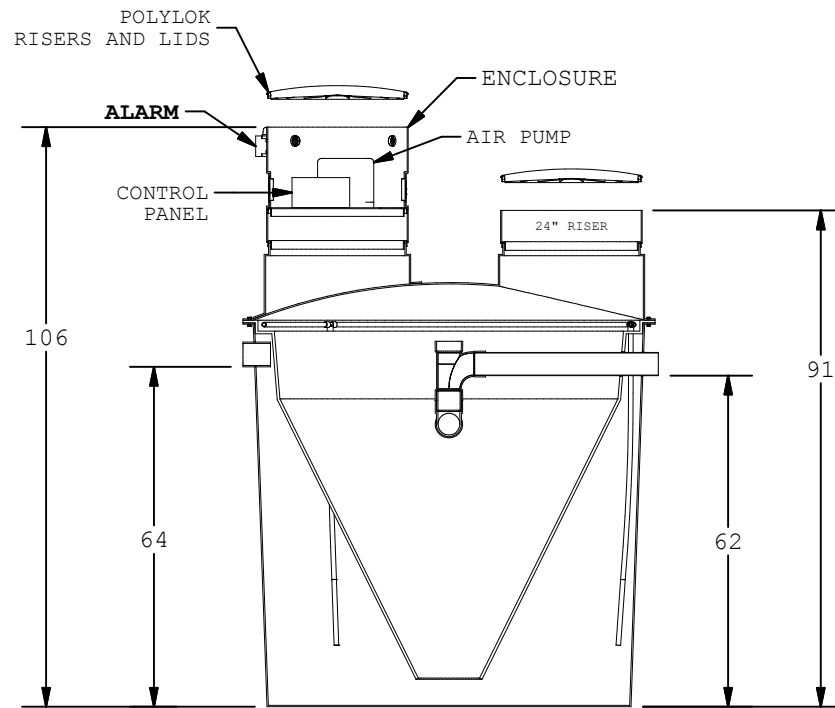
AERATION TANK
