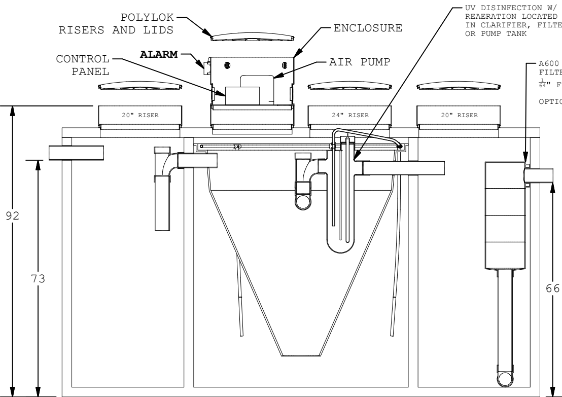
PRETREATMENT TANK
