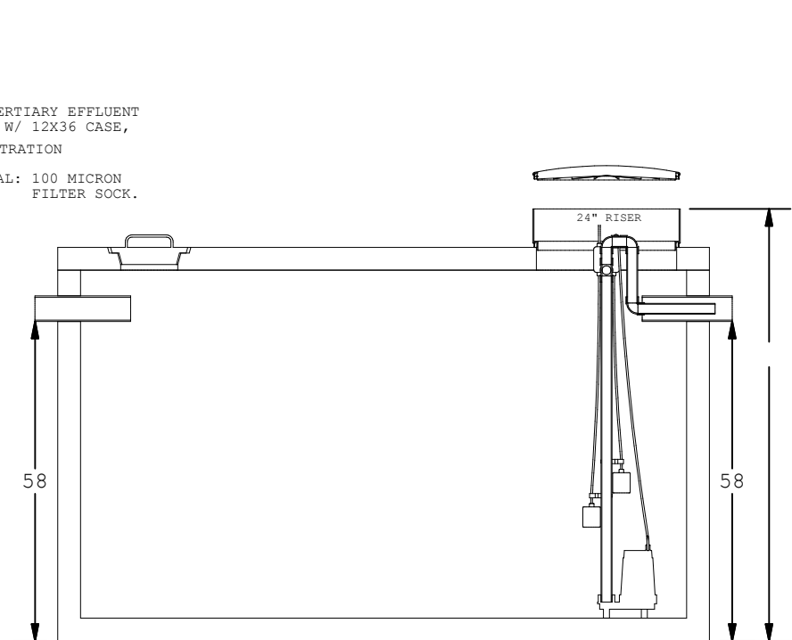
1500 GALLON PUMP TANK USA PRECAST PUMP TANK (13,000 lbs.)
