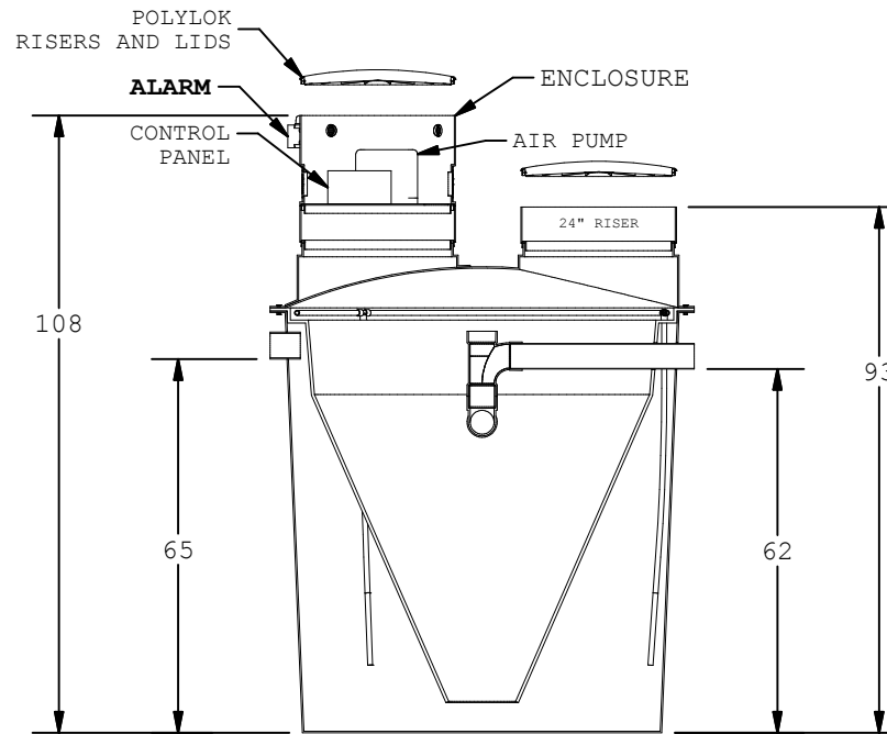
AERATION TANK
