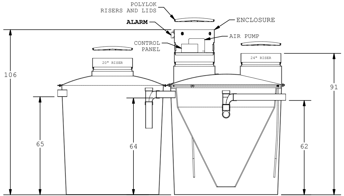
PRETREATMENT TANK
